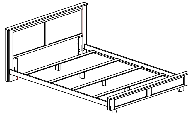
COMPLETED QUEEN BED ASSEMBLY
